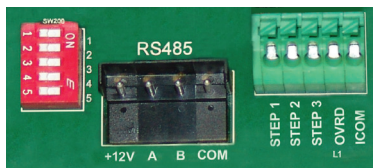
Figure 8: DIP Switches
