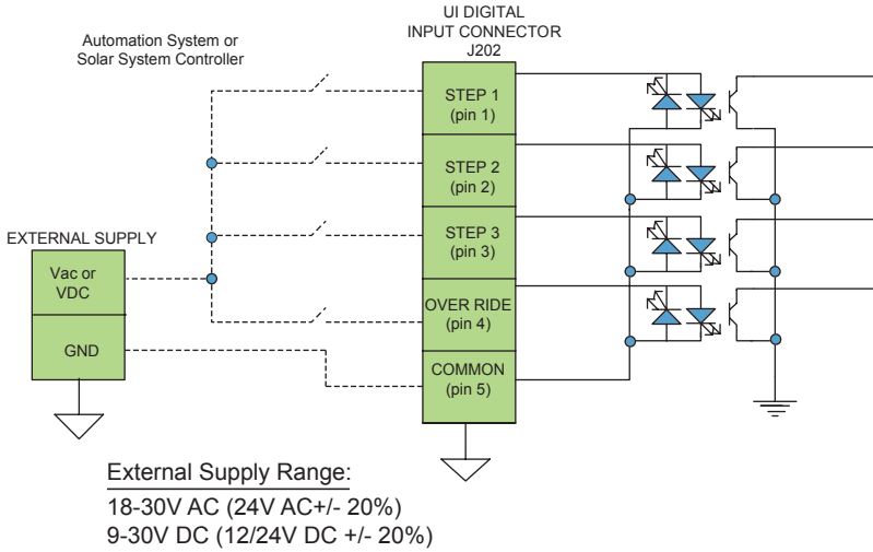
Figure 4: Wiring Diagram for Digital Inputs
