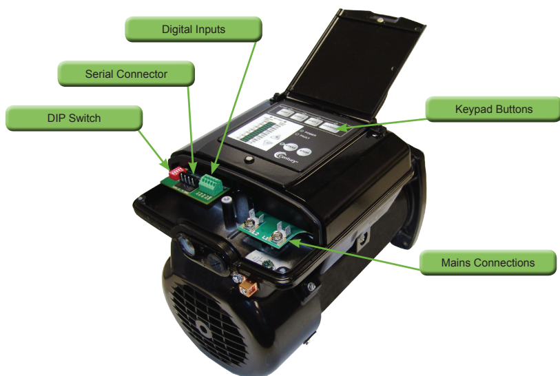
Figure 2: V-Green 165 Overview
