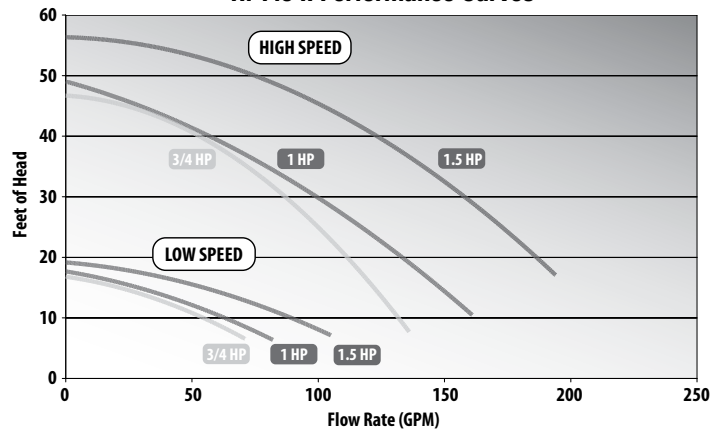
Hi-Flo II Performance Curves
