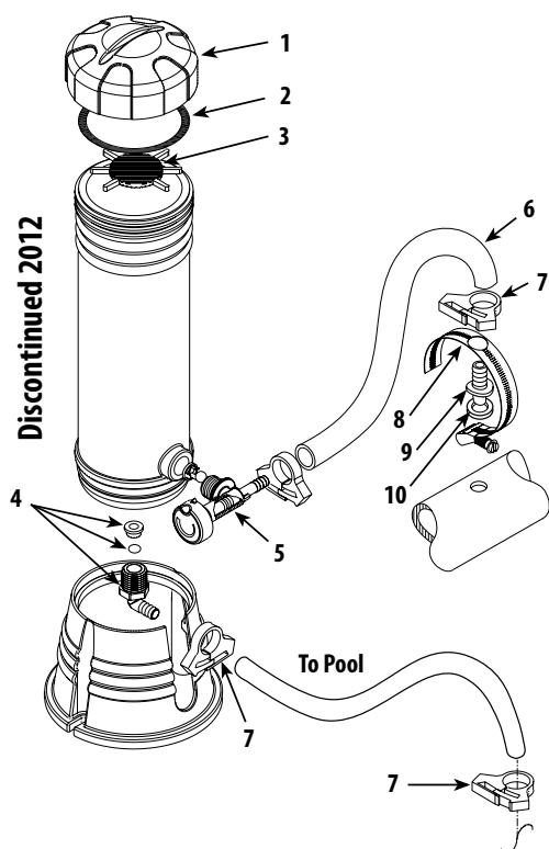
Off-Line Chlorinator
