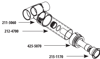
Tee Body Assembly
