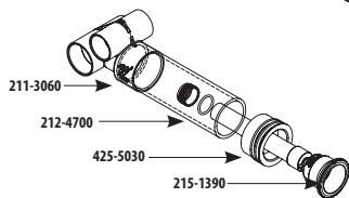
Tee Body Assembly
