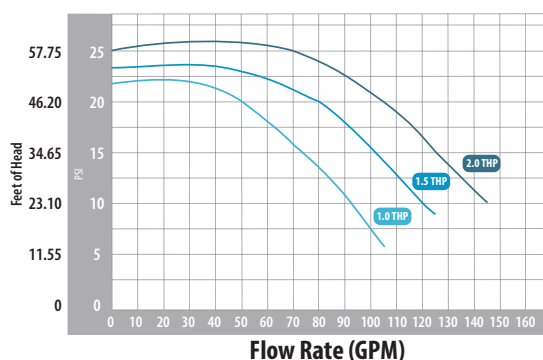
Spa-Flo II Flow Curves
