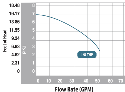
Iron Might Flow Curves
