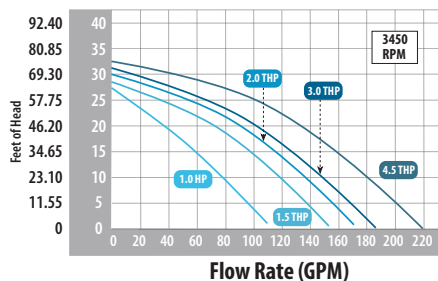
Executive 48-Frame Flow Curves
