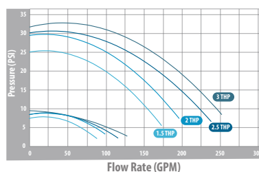
Executive 48-Frame Flow Curves
