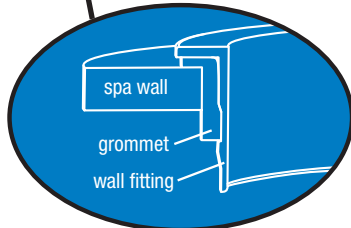
Sure-Grip Mounting System
