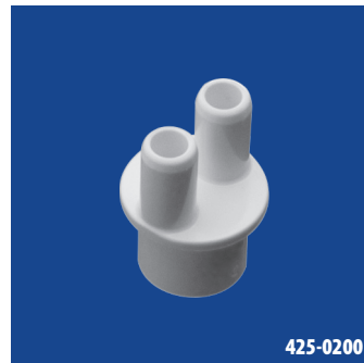
2-WAY ADAPTER (2) 3/8" SB x 1/2" SPG
