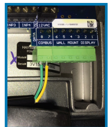
Figure 13. Pentair IntelliFlo/Hayward EcoStar Connection to Pump
