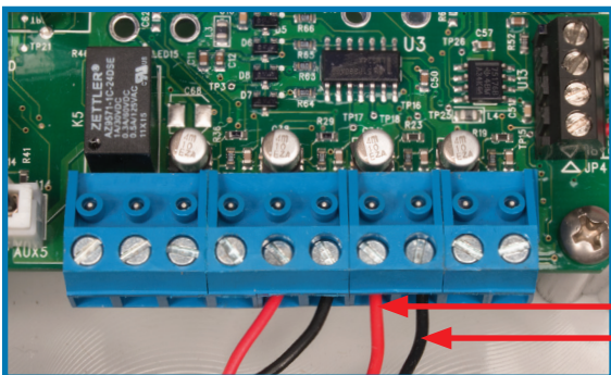
Figure 7. Sensor Connection
