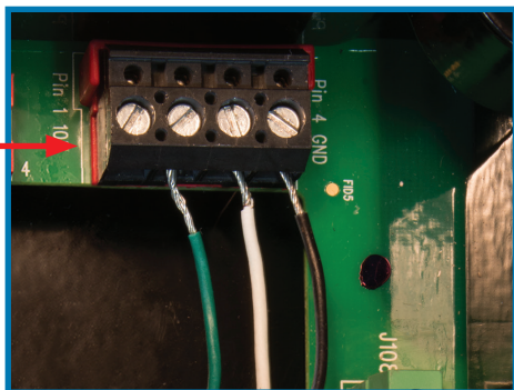
Figure 13. Pentair IntelliFlo/Hayward EcoStar Connection to Pump
