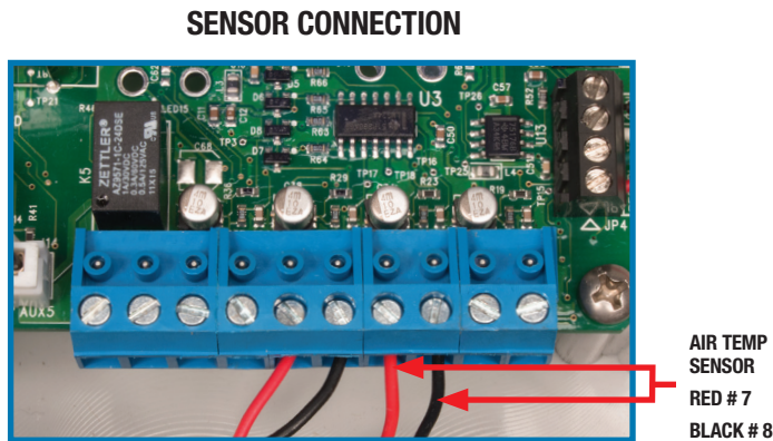
Figure 7. Sensor Connection
