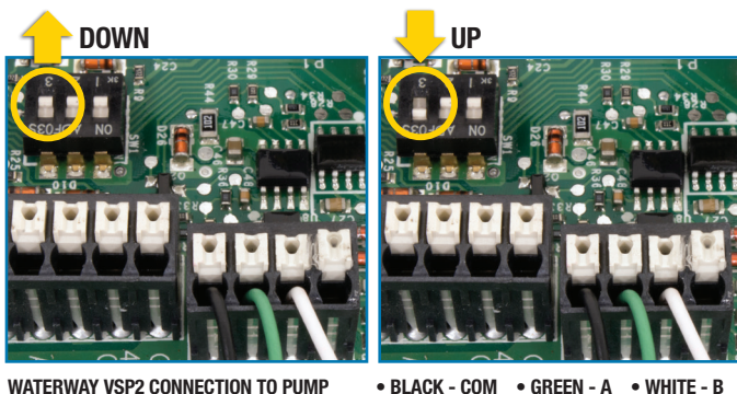
Figure 11.3 Note: Switch 3 must be moved to UP position before connection to Power Defender 300
