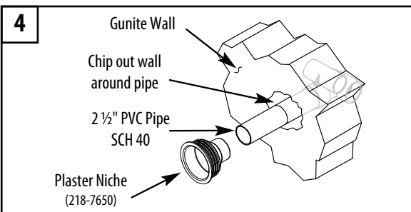
4. While guniting, scoop out gunite around the 2 1/2" PVC pipe, allowing for the plaster niche (218-7650). Before plastering, cut the 2 1/2" pipe so that the plastic niche will fit flush with the finished wall. Glue the plaster niche onto the pipe, then cover the niche with tape for plastering.
