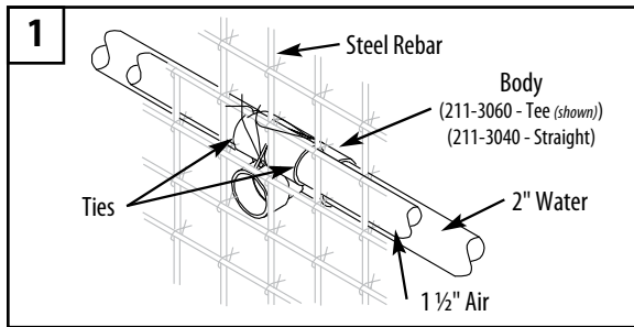
1. Hang Power Gunite Jet Body with ties through preset holes onto steel rebar.
