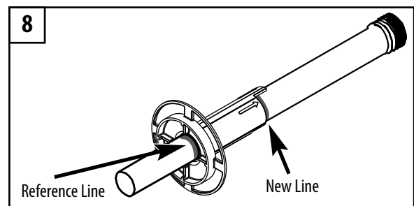
8. Remove the 1" pipe assembly from the jet body assembly and realign the measuring tool with the reference line. Make a new line at the Power Storm Gunite Jet setback on the measuring tool.
